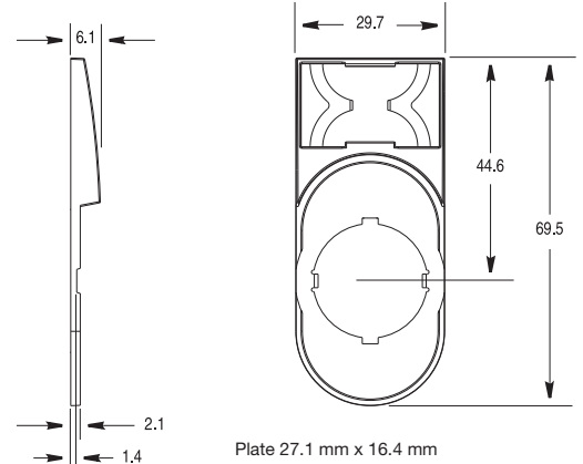
Special Multi-Function Snap-In Legend Plate
