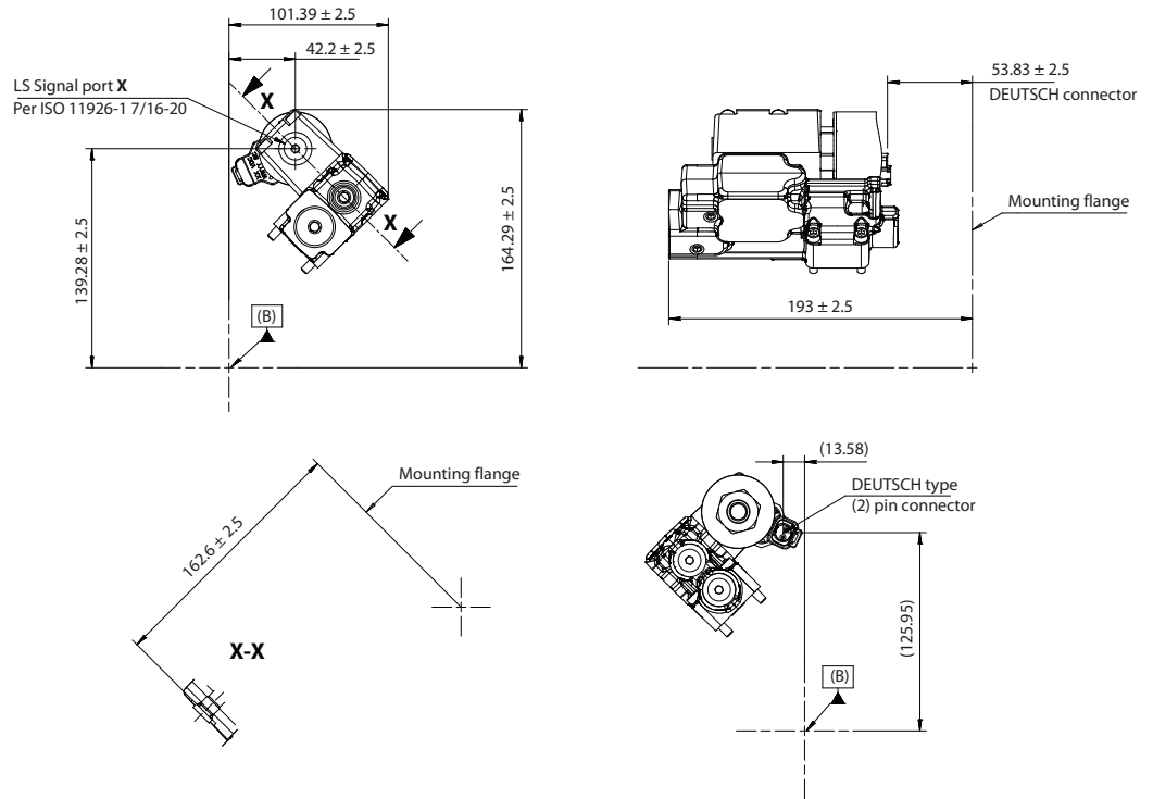
Single pool control, Left side
